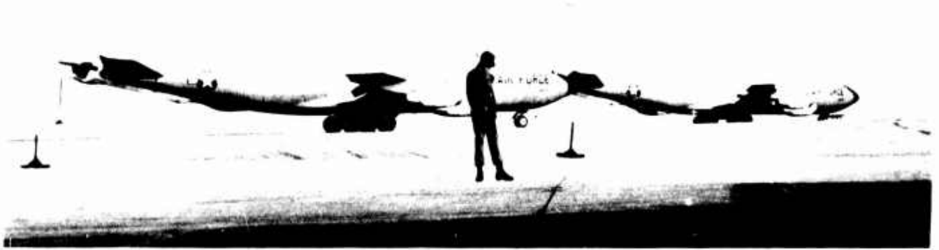
Drogue configured KC-135
