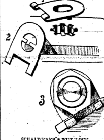
SCHAUWENKER'S NUT LOCK. Fig. 2 representing the blank of the lock plate as it is punched out...
