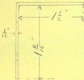
IRON BRACKET Make 36
